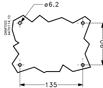
Drilling dimensions
