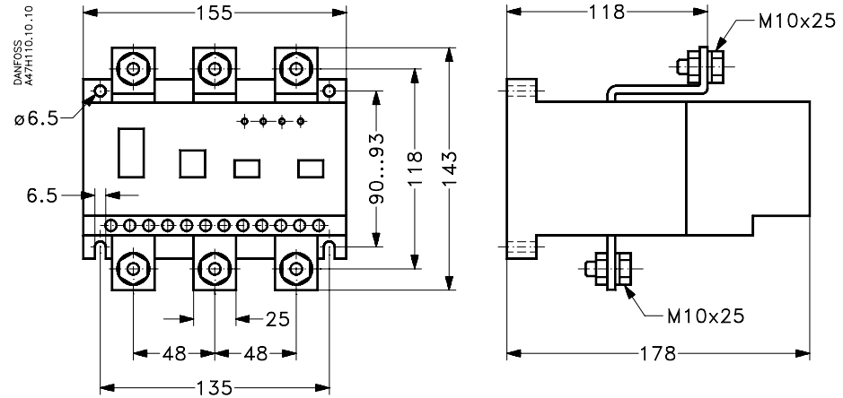
Electronic motor protection relay TI 630 E
